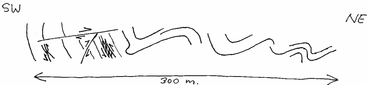
Figure 20. Sketch of outcrop in STOP 11.
