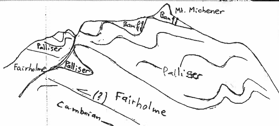
Figure 22. View to Mt. Michener from Windy Point (STOP 12) with sketch of geology.
