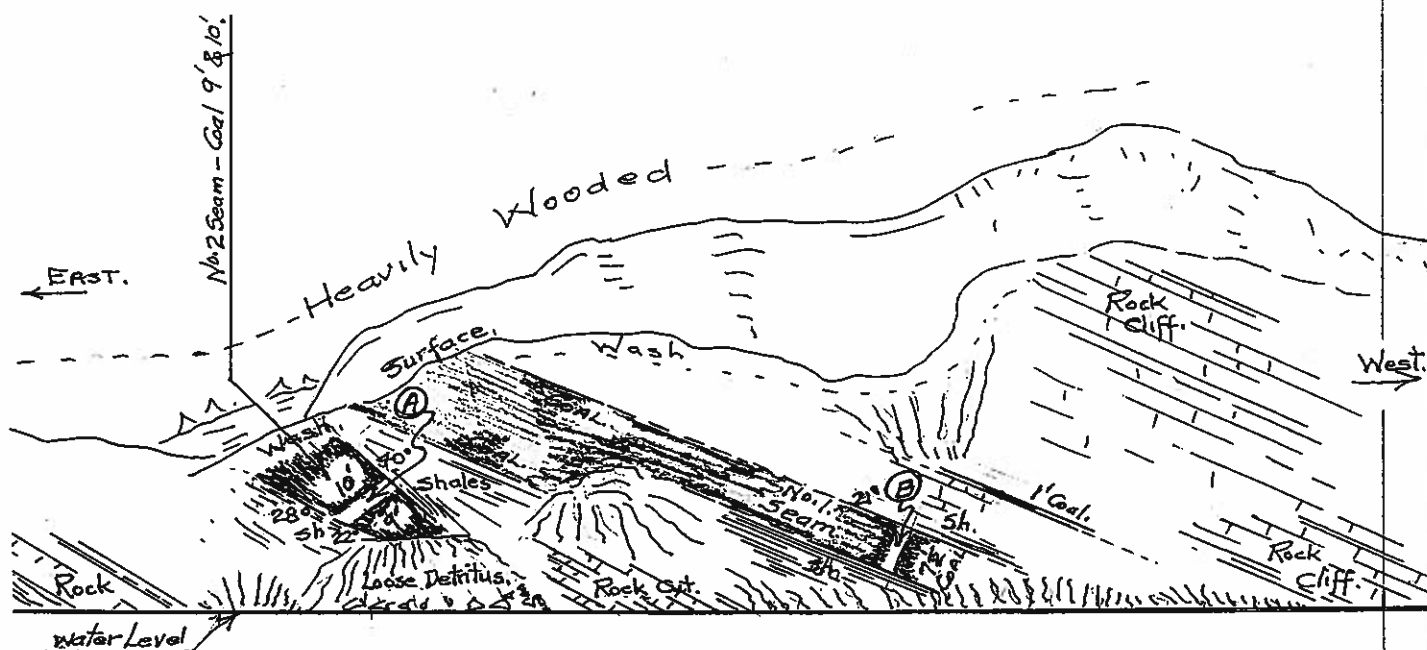
ELEVATION OF SOUTH BANK OF BIGHORN RIVER. at about point marked Prospect, Sec. 27. T. 39 R. 17 on Nordegg Sheet - Map. 302A. showing location of Channel Samples A & B. May. 22. 1959. N.M.
