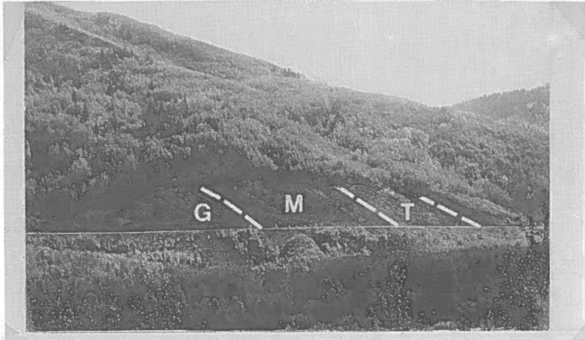
Figure 10. Overview of the section of Stop 2. Gladstone Formation (G) at the bottom, Moosebar Formation (M) in middle and Torrens Member (T) at the top.
