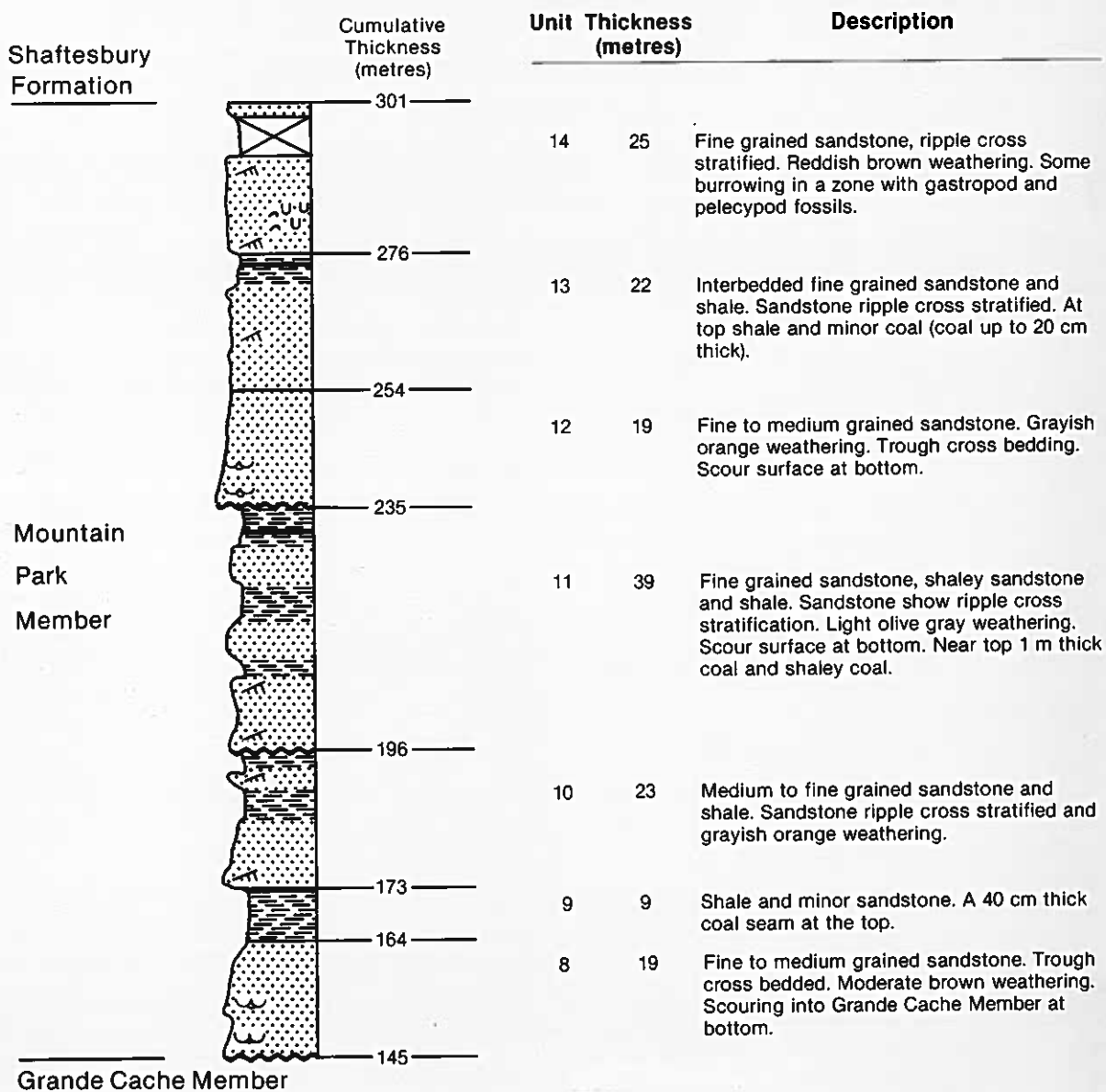
Figure 13. Columnar stratigraphic section of the Mountain Park Member in Stop 3.
