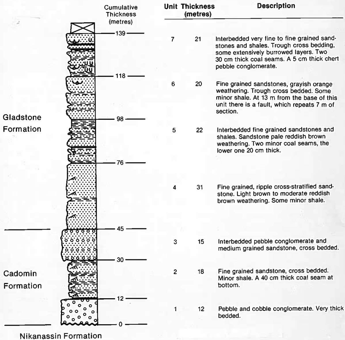
Figure 6. Columnar stratigraphic section of the Cadomin and Gladstone Formation in Stop 1.
