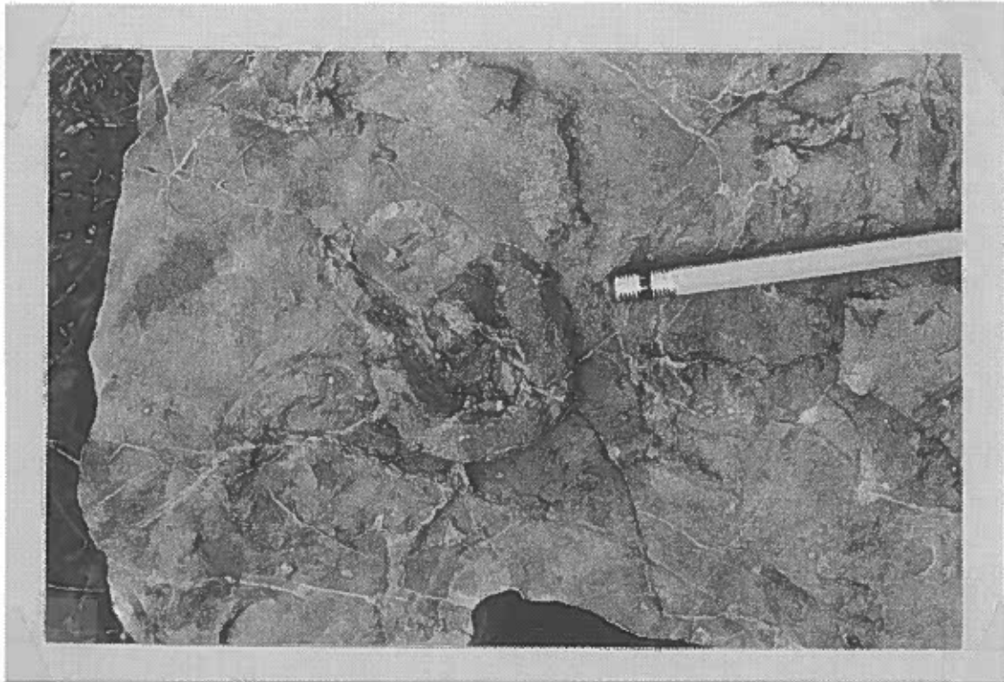
Figure 8. The trace fossil Diplocriterion in the upper Gladstone Formation of Stop 1.
