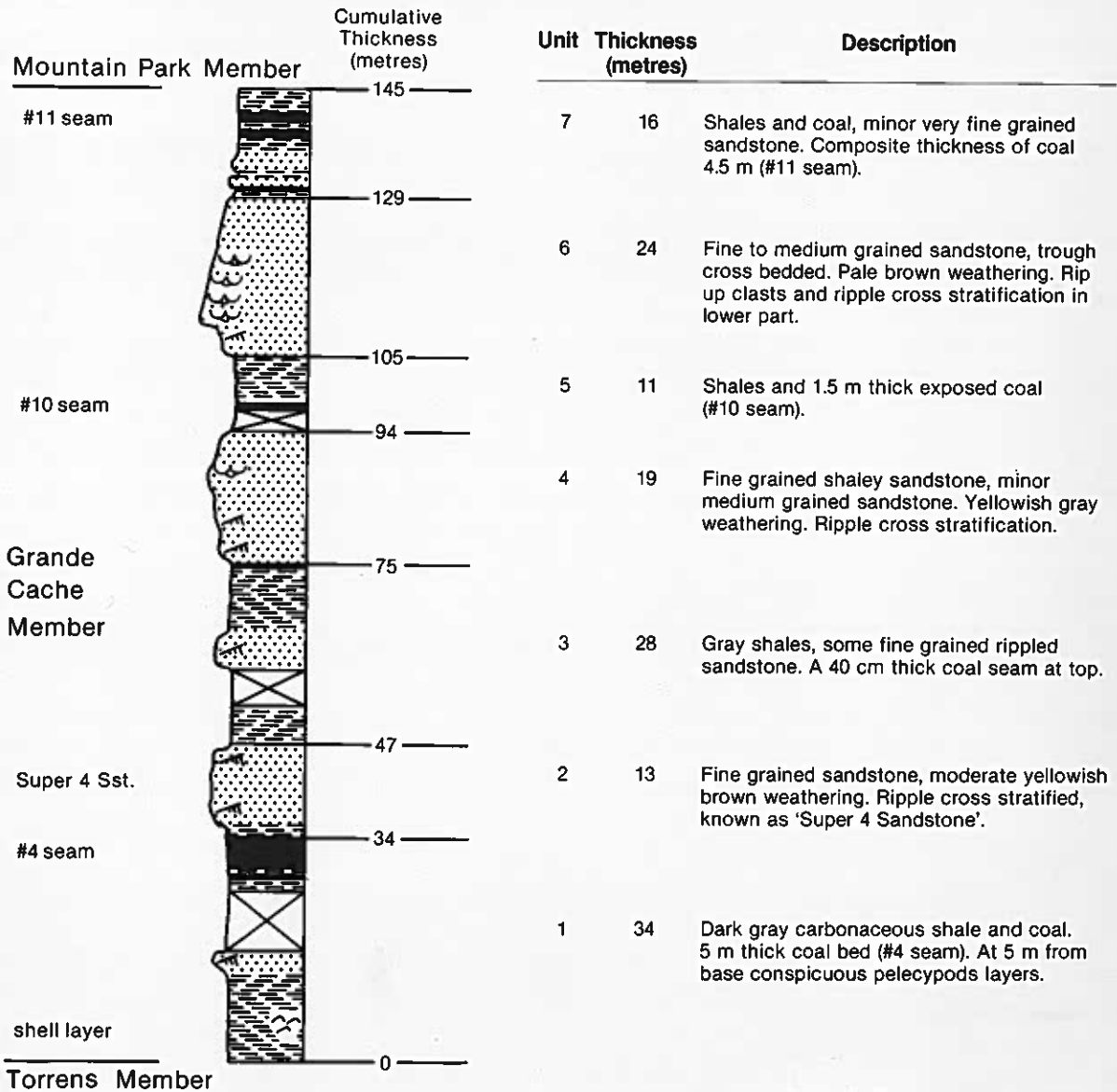
Figure 12. Columnar stratigraphic section of the Grande Cache Member in Stop 3.
