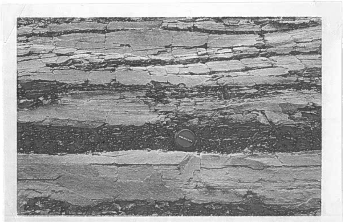
Figure 11. Hummocky cross-beds in the upper part of the Moosebar Formation of Stop 2.
