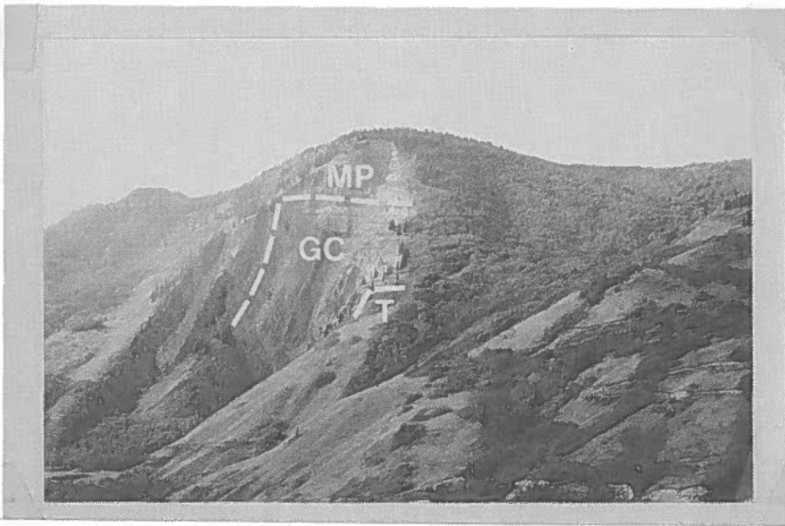
Figure 15. Chevron fold across the Smoky River from Stop 3. T = Torrens Member, GC = Grande Cache Member, MP = Mountain Park Member.
